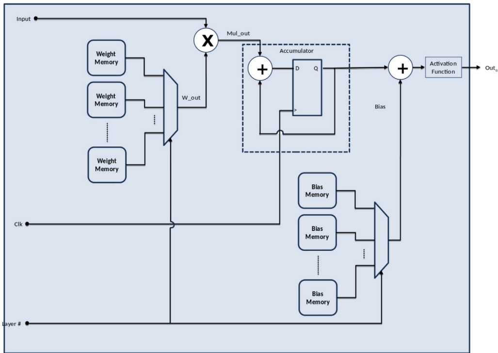
Fig. 7. Internal architecture of a hardware-implemented Neuron used in dense layers. Each neuron performs fixed-point multiply-and-accumulate (MAC) operations by reading input activations and weights from on-chip memory. The design supports efficient reuse across multiple dense layers through a layer selection signal (layer #), which dynamically controls memory multiplexing.
