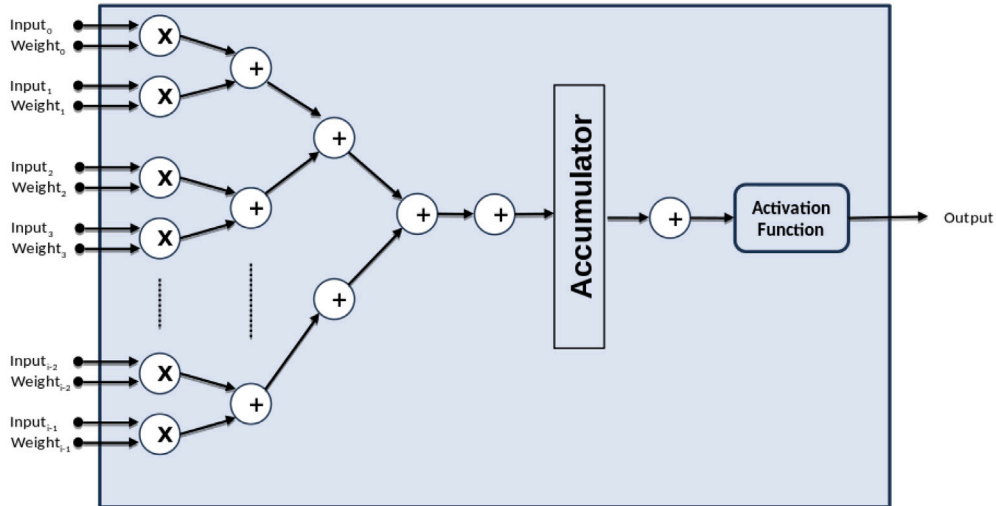
Fig. 5. Detailed architecture of the Kernel Module implementing MAC and activation logic. The module computes the element-wise multiplications between input values and kernel weights using a partially parallel structure optimized for low-cost FPGAs. The products are summed using a tree-based adder.
