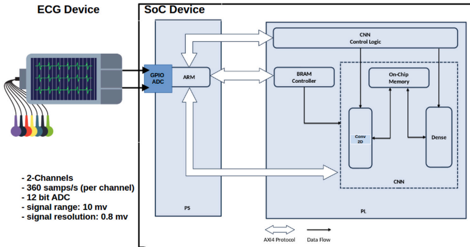
Fig. 1. Overall system architecture.
