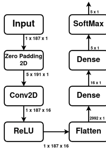
Fig. 8. Structure of CNN model.
