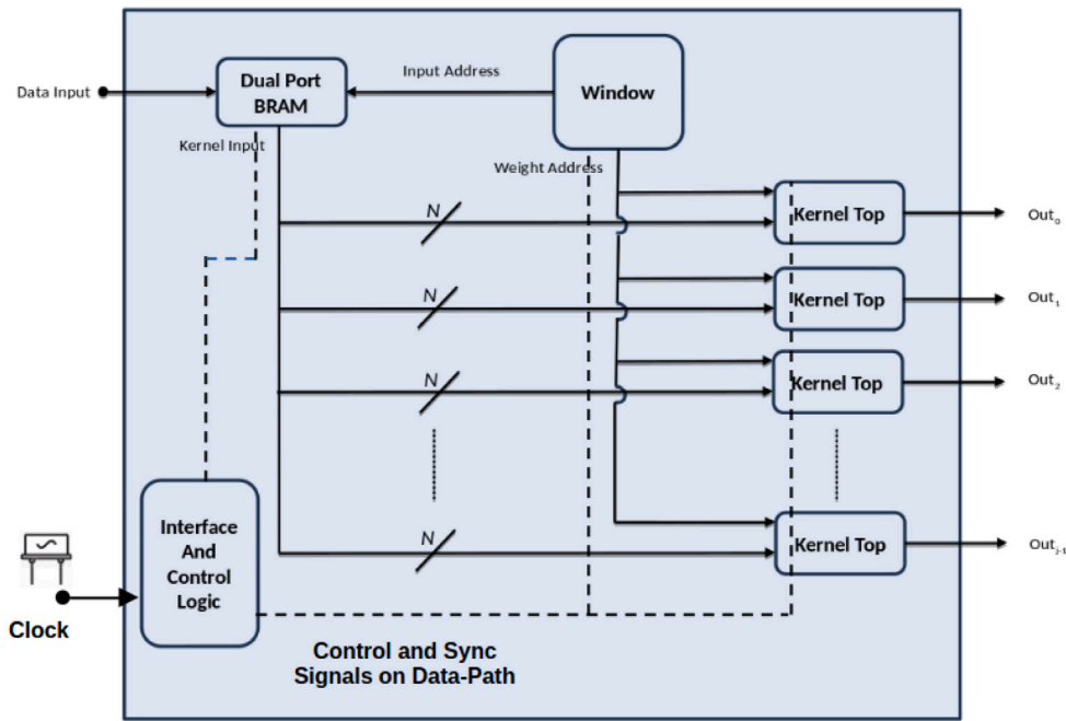
Fig. 3. Hardware architecture of the Conv2D layer accelerator optimized for FPGA implementation. This design integrates key modules to perform efficient 2D convolution on ECG signal data.
