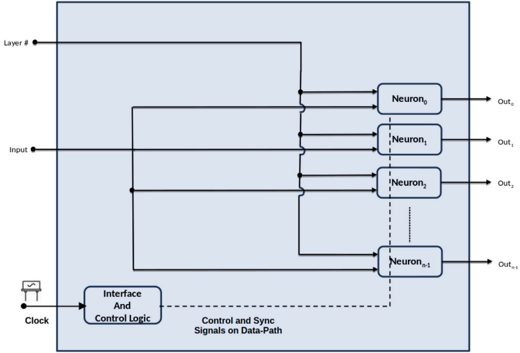
Fig. 6. Hardware implementation of a scalable Dense (Fully Connected) Layer. This architecture supports multiple dense layers and dynamically enables neurons depending on the active layer configuration. Each neuron performs fixed-point MAC operations followed by bias addition and activation.
