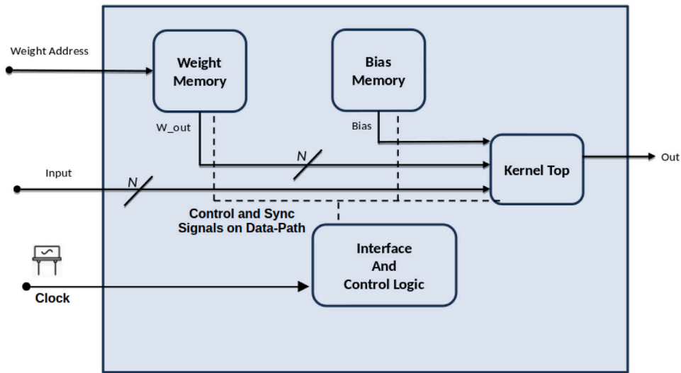
Fig. 4. Structure of the Kernel Top Module responsible for convolution execution. It performs the core multiply-and-accumulate (MAC) operations of the convolution layer by fetching input windows and corresponding kernel weights in parallel. It supports address computation, weight selection, and bias retrieval.
